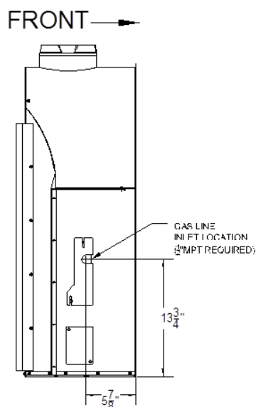
Figure 3-20 Gas Line Inlet Location
