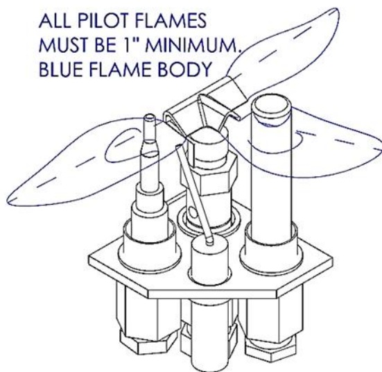
Figure 4-10 Pilot Flames
