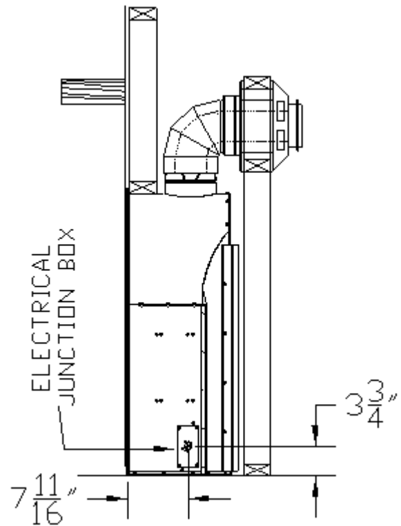
Figure 3-17 Electrical Junction Box
