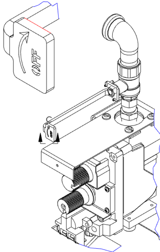
Figure 3-24 MANUAL GAS SHUTOFF
