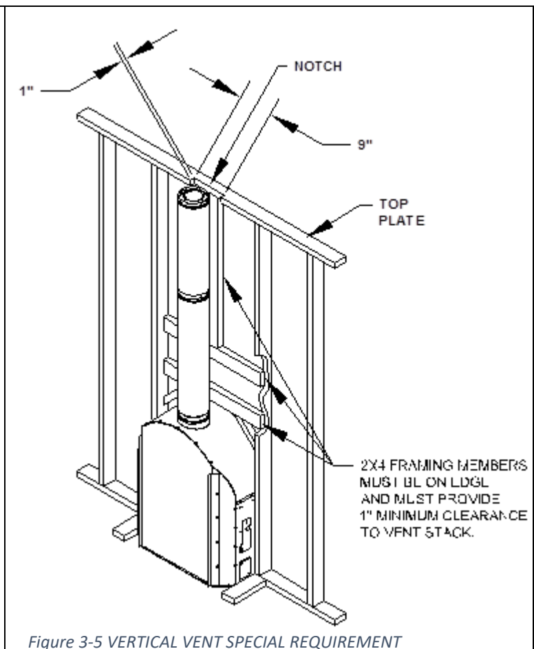
Figure 3-5 VERTICAL VENT SPECIAL REQUIREMENT
