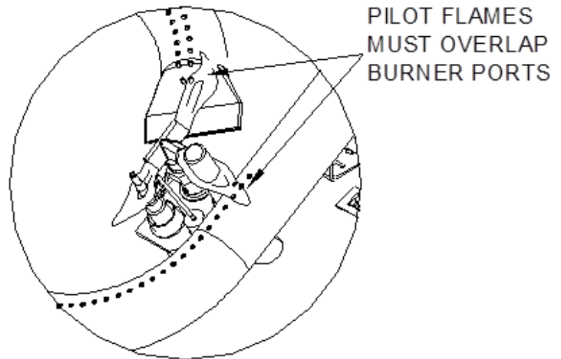
Figure 4-11 Pilot Flame and Burner Ports
