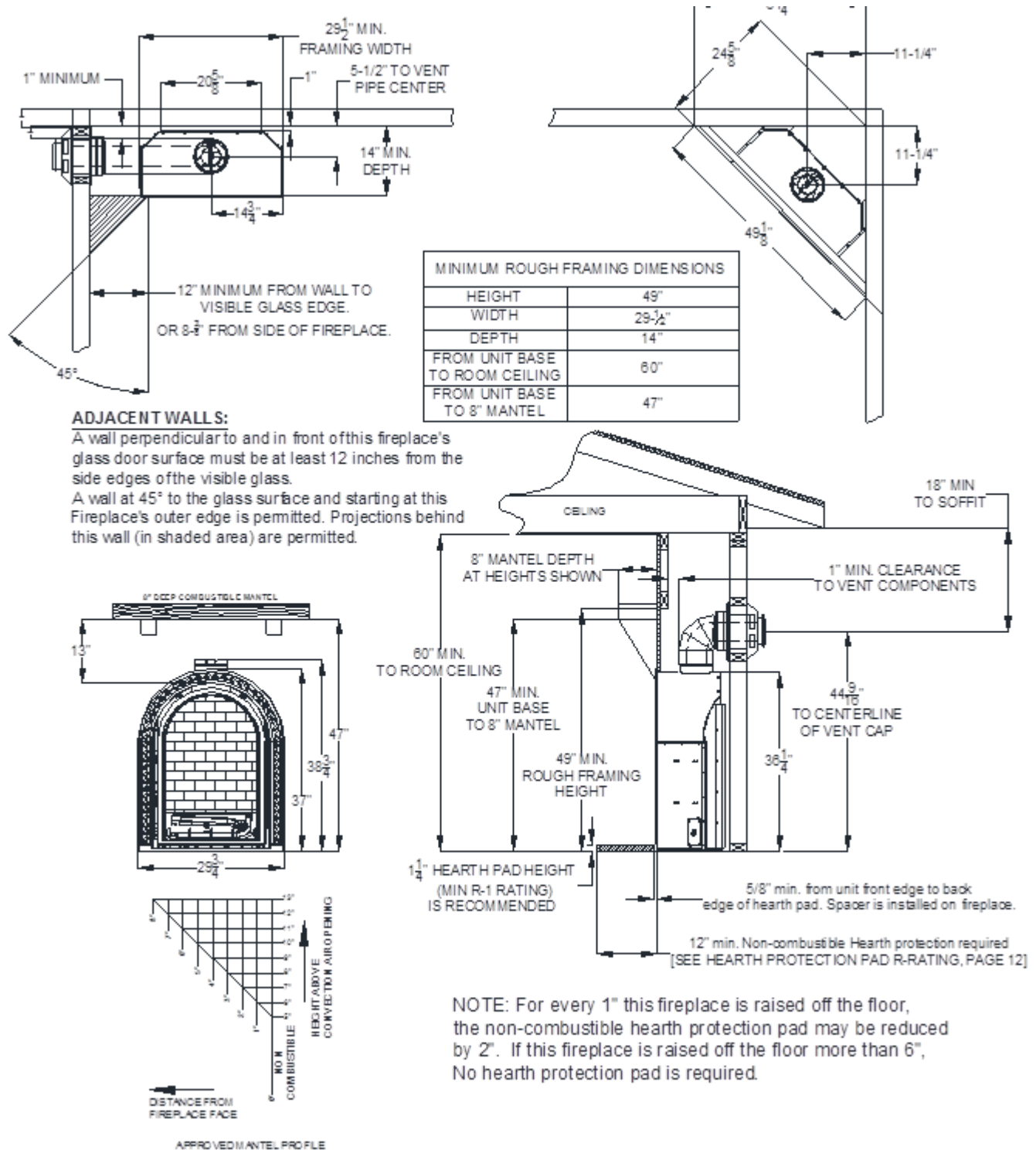
Figure 3-3 Overall Fireplace Dimensions
