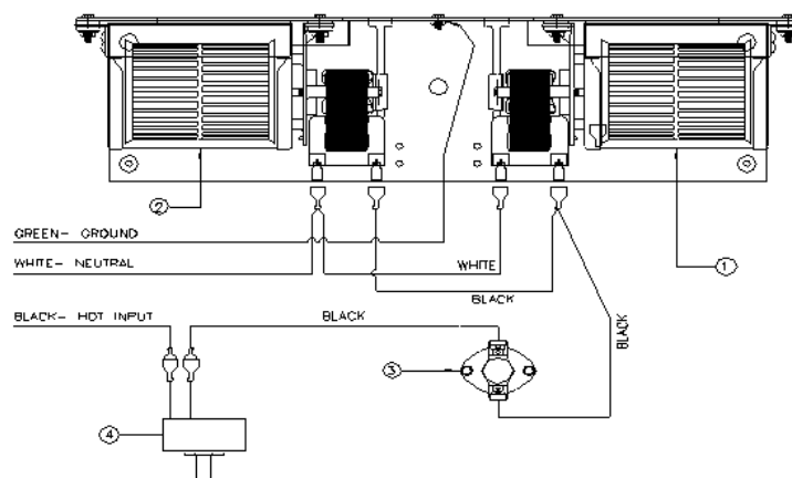
Figure 3-19 BLOWER CIRCUIT DIAGRAM
