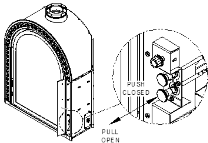
Figure 4-12 Burner Air Shutter Controls
