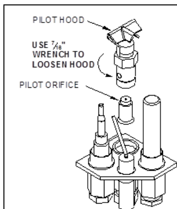
Figure 4-8 Pilot Orifice
