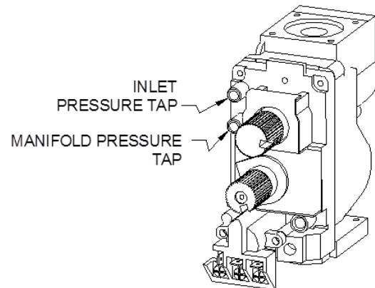
Figure 3-21 Main Gas Valve
