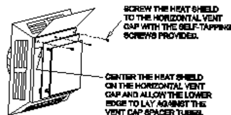
Figure 3-15 WALL HEAT SHIELD
